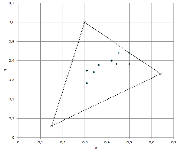
a b Fig. 2, Patches xy coordinates in: a – headlight gamut [AFN1], b – sRGB gamut
