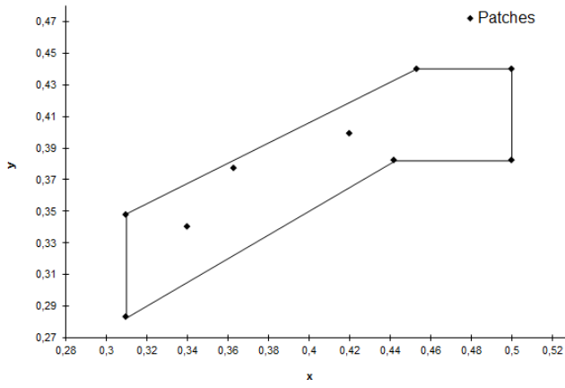
a b Fig. 2, Patches xy coordinates in: a – headlight gamut [AFN1], b – sRGB gamut
